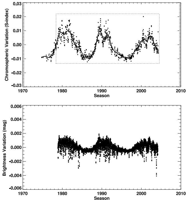
FIG. 2.—Ca II K and total irradiance variability of the Sun. The K data are from White et al. (1998) plus updates from W. C. Livingston (2007, private communication). The irradiance data (Fröhlich 2003a, 2003b) can be found at http://www.pmodwrc.ch/pmod.php?topic=tsi/composite/SolarConstant (graph) or http://www.ngdc.noaa.gov/stp/SOLAR/IRRADIANCE/irrad.html (links to tabular data).
